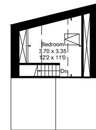
Annexe - First Floor Area = 15.3 sq m / 165 sq ft (Limited Use Area = 8.4 sq m / 90 sq ft)
