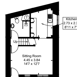
Annexe - Ground Floor Area = 29.1 sq m / 313 sq ft (Not Shown In Actual Location / Orientation)
