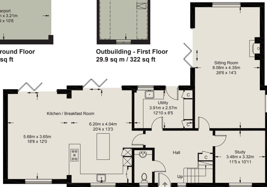
Ground Floor 130.1 sq m / 1400 sq ft
