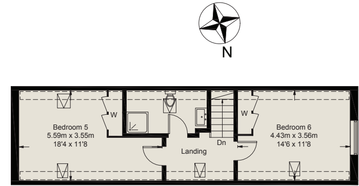
Second Floor 46.0 sq m / 495 sq ft
