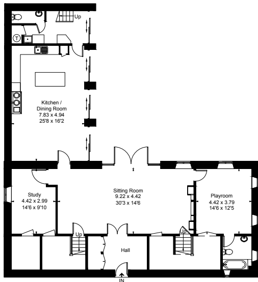
Ground Floor Area = 167.5 sq m / 1803 sq ft (Limited Use Area = 19.3 sq m / 208 sq ft)
